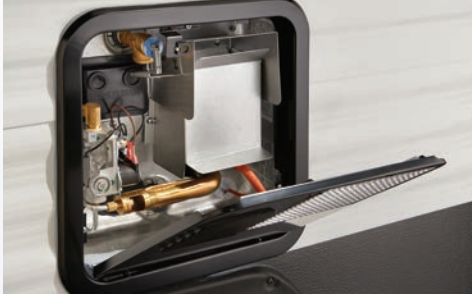
Six gallon gas/electric direct start ignition (DSI) water heater
